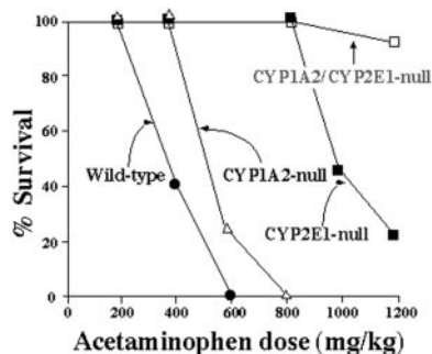
Fig. 1. Acetaminophen toxicity in wild-type, CYP1A2-null, CYP2E1-null, and CYP1A2/CYP2E1-double-null mice. Mice were administered acetaminophen, and the number of mice surviving at 48 h later was determined. Data are redrawn and combined from Zaher et al. (1998).
