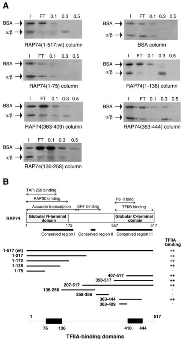
FIG. 4. Interactions of TFIIA \alpha/\beta with RAP74 deletion mutants. A, protein affinity chromatography was performed using columns containing immobilized RAP74 fragments (wild type or deletions mutants). A volume of 50 \mu l containing 200 ng of TFIIA \alpha/\beta was chromatographed through each column. Fractions were collected and analyzed as in Fig. 2. The positions of TFIIA \alpha/\beta and BSA (as an internal negative control) are indicated. B, summary of the interactions between the RAP74 deletion mutants and TFIIA. The various domains of RAP74 are indicated in the top part. The two TFIIA-binding domains of RAP74 are deduced from our analysis.
