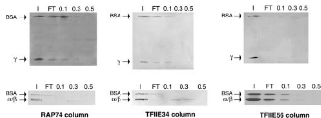
FIG. 3. Interactions of TFIIA \alpha/\beta and TFIIA \gamma with RAP74, TFII E56, and TFII E34. Protein-affinity chromatography was performed using microcolumns containing immobilized RAP74, TFII E34, and TFII E56. A volume of 50 \mu l containing 200 ng of TFIIA \alpha/\beta and TFIIA \gamma was chromatographed through each column. Fractions were collected and analyzed as in Fig. 2. The positions of \alpha/\beta , \gamma , and BSA (as an internal negative control) are indicated.
