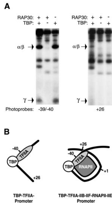
FIG. 1. Photo-cross-linking of rTFIIA on the AdMLP. A, photo-cross-linking experiments with photoprobes -39/-40 and +26 were performed in the presence of rTFIIA ( \alpha/\beta and \gamma ), TBP, TFIIB, TFIIF (RAP74 and RAP30), TFIIE (p56 and p34), and RNAPII. The specificity of the cross-linking signals was assessed by comparing reactions performed with all the factors to ones performed in the absence of TBP. Under our reaction conditions, the absence of TBP has the same effect as the use of a photoprobe with a mutation in the TATA element (TATAAAA to TAGAGAA) (55). The position of TFIIA \alpha/\beta and TFIIA \gamma are indicated. B, schematic representation of promoter contacts by TFIIA in the context of the TBP-TFIIA-promoter complex and the TBP-TFIIA-TFIIB-TFIIF-RNAPII-TFIIE-promoter complex in which the DNA adopts a wrapped structure. Positions -39/-40 , +26 and +1 are indicated. Only TBP, TFIIA, and RNAPII are represented to simplify the diagram.
